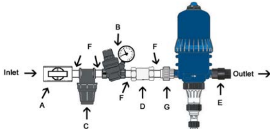
IPK34 - 10 GPM Industrial Plumbing Kit
