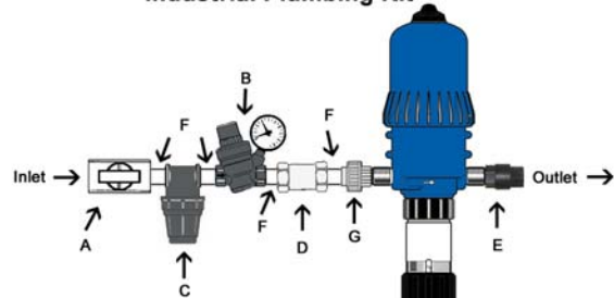
IPK34 - 7 GPM Industrial Plumbing Kit
