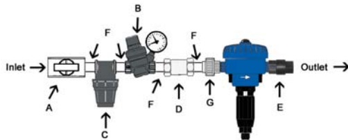
IPK34 - 3 GPM Industrial Plumbing Kit
