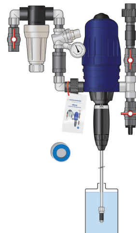
IPK34 - 7 GPM Industrial Plumbing Kit
